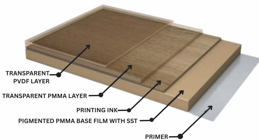
STRUCTURE OF EXTERIOR FILM-RENOLIT EXOFOL FX
