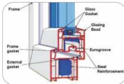
GALVANIZED REINFORCEMENT FOR uPVC DOORS & WINDOWS
