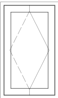
VERTICAL PIVOT LEFT HAND OPENING
