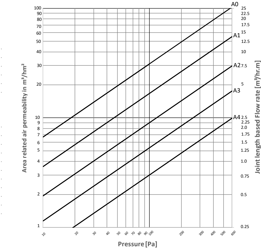
FIG. 6A CLASS A — GRAPH TO PLOT ACTUAL FLOW RATES OF THE SPECIMEN
