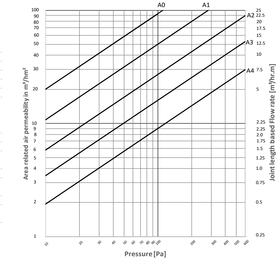
FIG. 6B CLASS B — GRAPH TO PLOT ACTUAL FLOW RATES OF THE SPECIMEN
