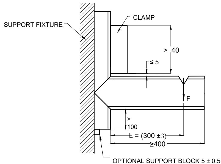
FIG.7 EXAMPLE OF A TEST RIG FOR A TENSILE BENDING TEST OF CORNERS
