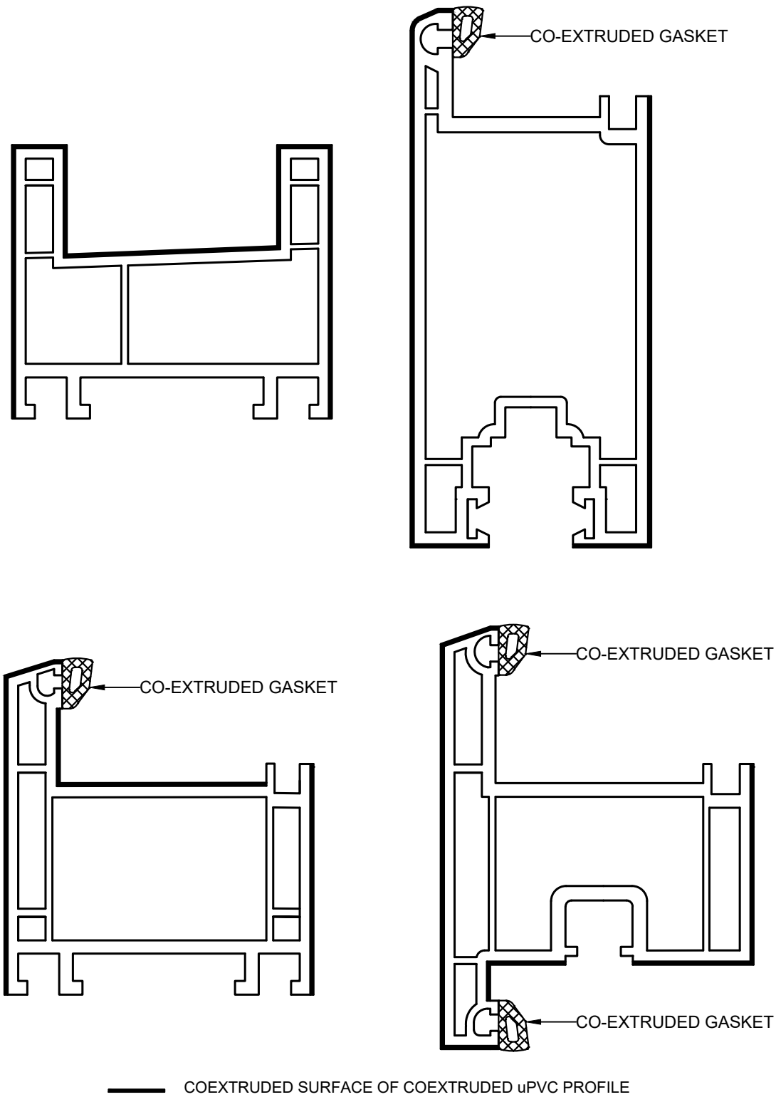
FIG. 2 EXAMPLES OF TYPICAL COEXTRUDED PROFILES
