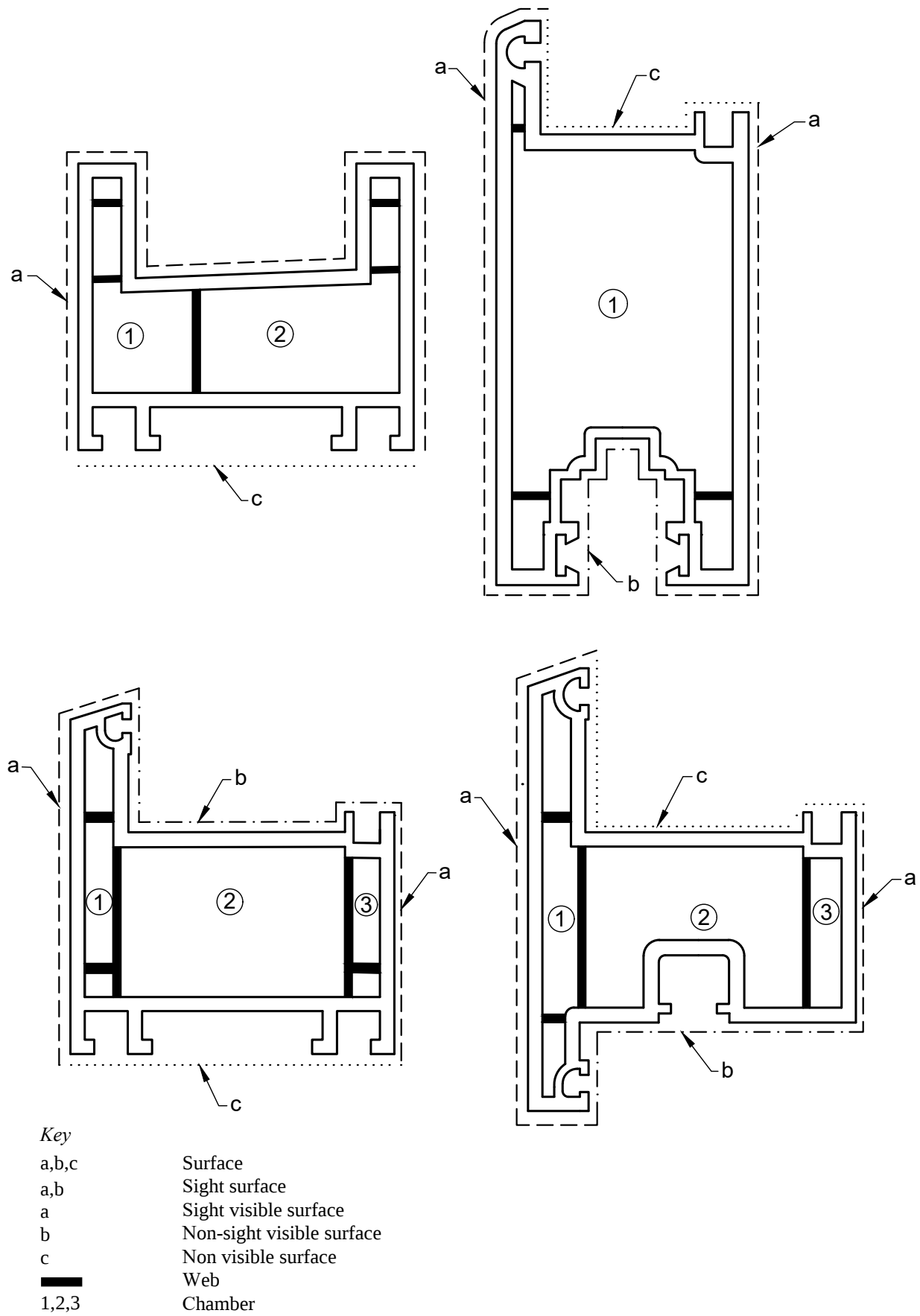
FIG. 1 SURFACE, WEB AND CHAMBER IN DIFFERENT TYPE OF PROFILES
