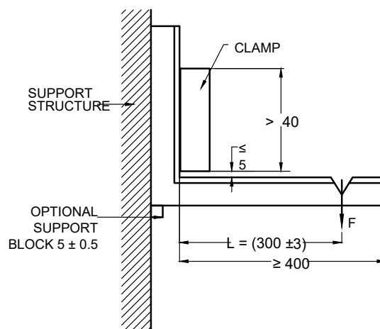
FIG.7 EXAMPLE OF A TEST RIG FOR A TENSILE BENDING TEST OF CORNERS
